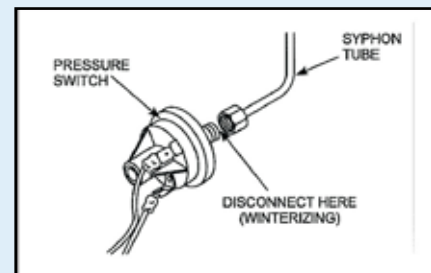
PRESSURE SWITCH
