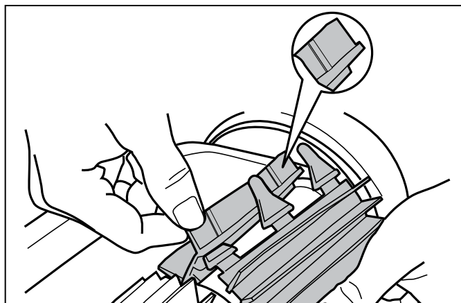
Figure 29. Wear Indicators
