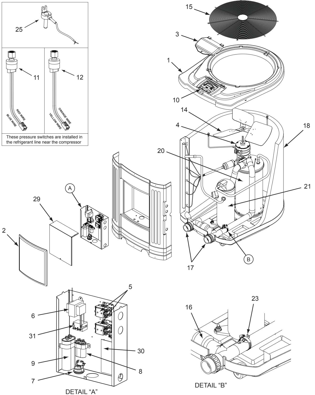
Figure 18. Jandy AE-Ti Heat Pumps Exploded View
