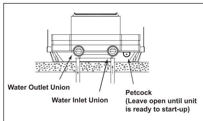
Figure 16. Winterizing the AE-Ti Heat Pump
