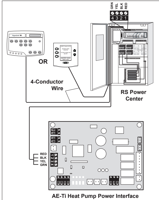
Figure 14. AE-Ti Heat Pump Connection to Power Center
