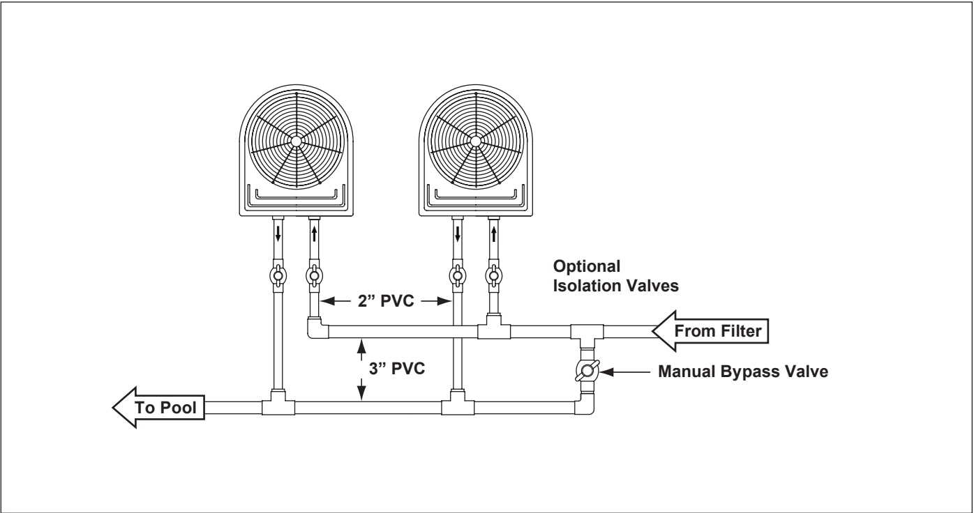
Figure 6. Two Heat Pump Plumbing Layout
