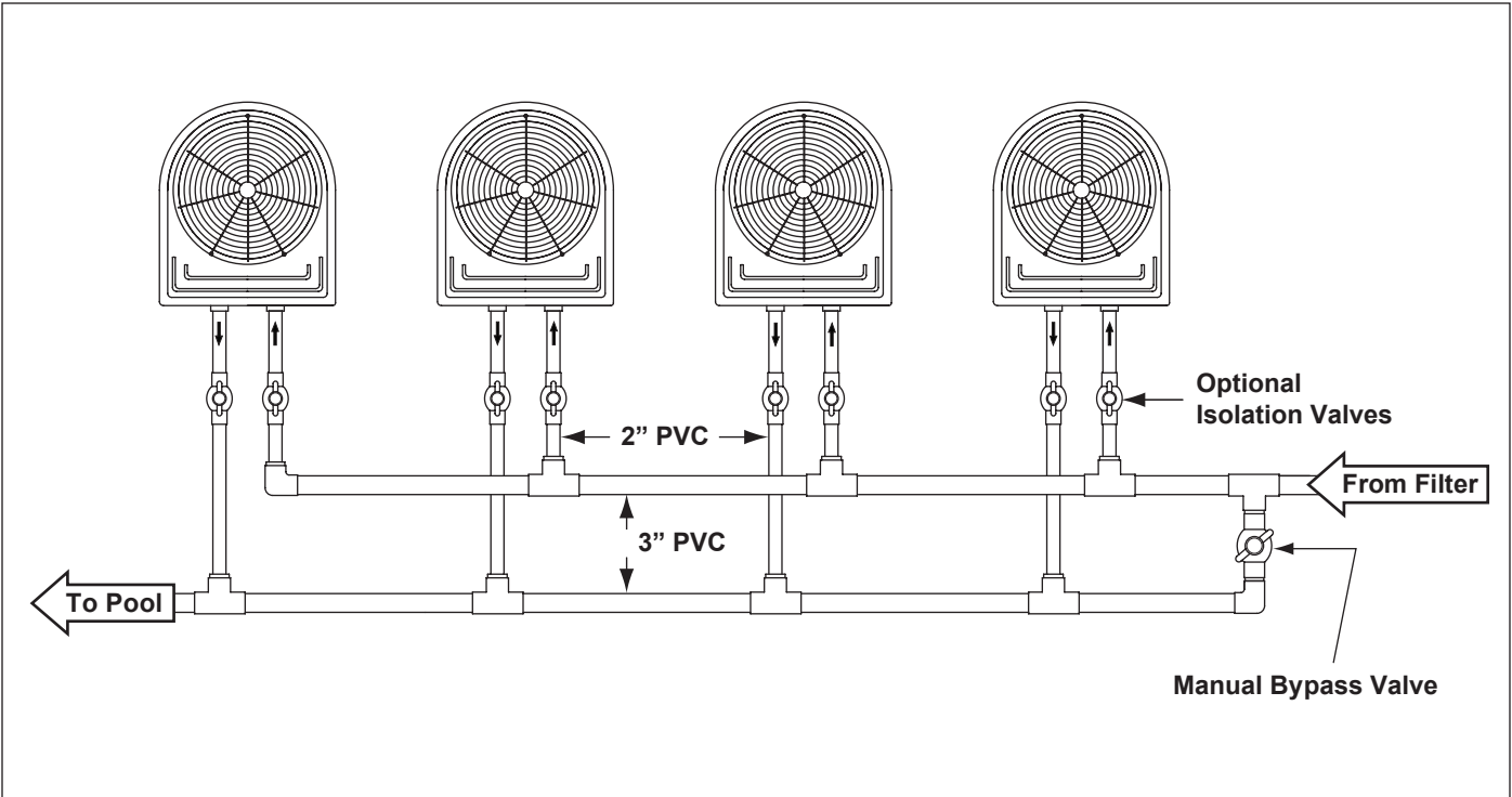
Figure 7. Four Heat Pump Plumbing Layout
